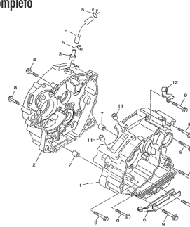
TAV.8 Carter motore - Crankcase assy. - Carter moteur complet - Kurbelgehäuse, compl. - Carter motor completo
